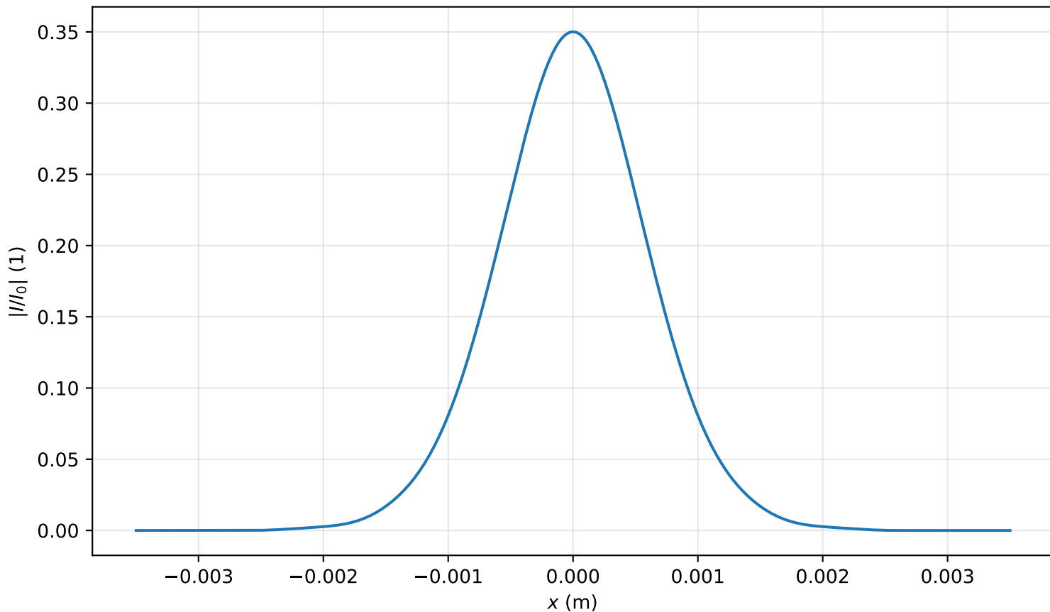
Intensity profile I(x, y = 0, z = 3.821m)/I_0 , P_{in}=0.4P_{cr} , artificial time
